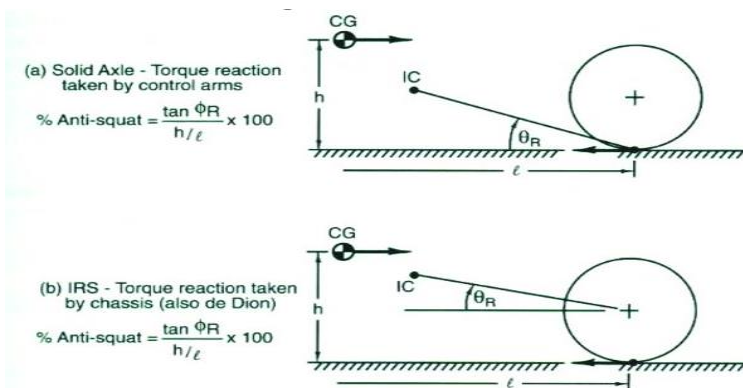
Figure 10: The Anti-Squad Geometry and its characterization
