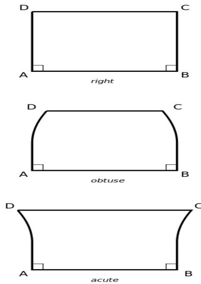
Figure 9: A Saccheri quadrilateral and its representation
