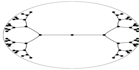
Figure 12: The characterization of Citation and its graphical visualization in one frame
