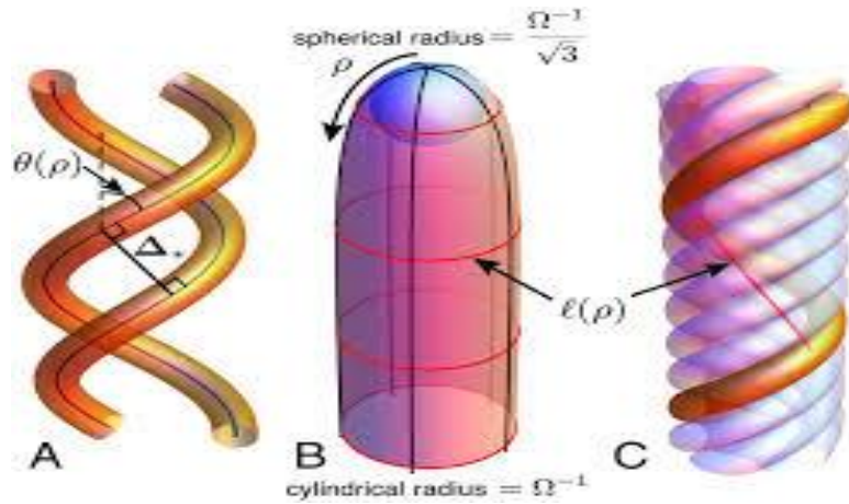
Figure 8: One of the applications of Non-Euclidean Geometry i.e. Twisted bundles
