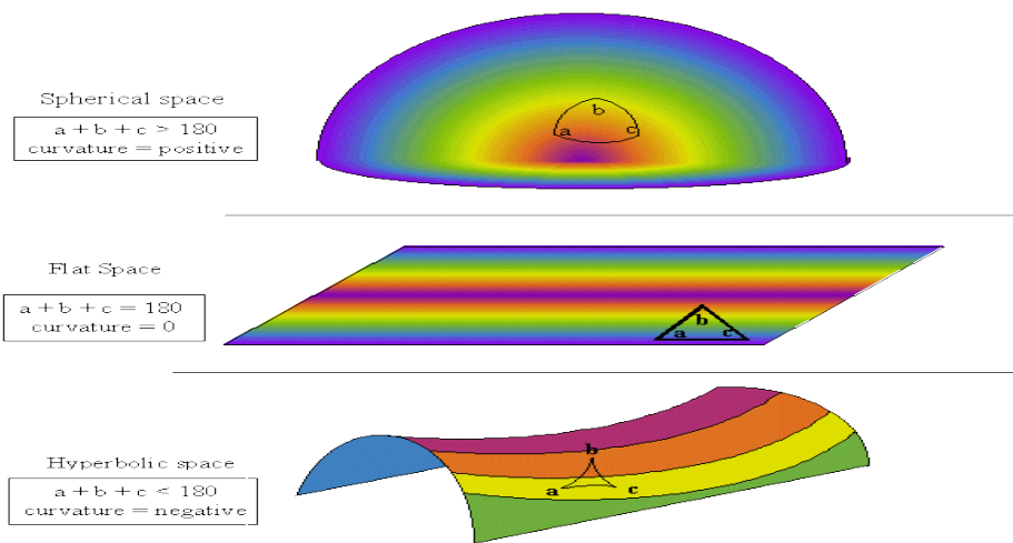
Figure 6: The difference between Euclidean and Non-Euclidean data sets and its representation
