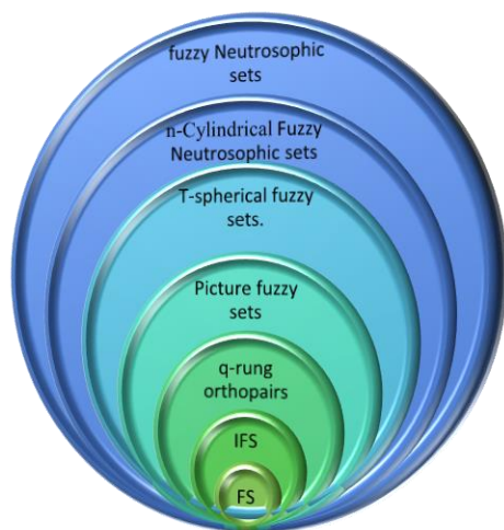
Figure: 4: Hierarchy of Fuzzy extensions.
