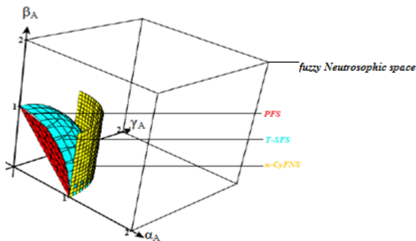
Figure 2: Comparison between n-CyFNS, T-SFS & PFS spaces.
