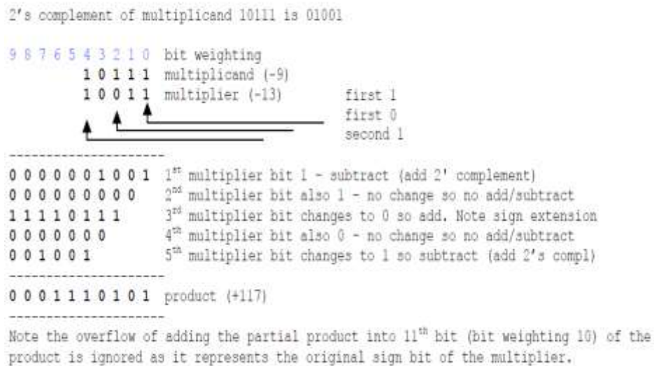
Figure 5: Explanation of Booth multiplication algorithm
