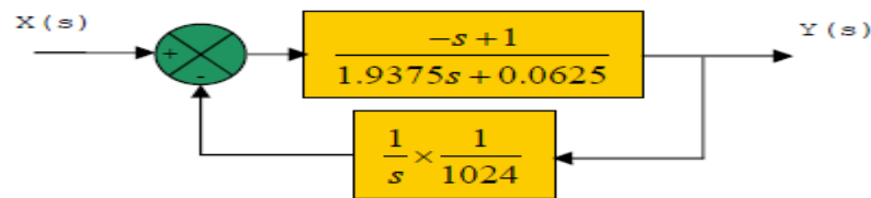
Figure 10: Block diagram of PLL system in analyzing transient response
