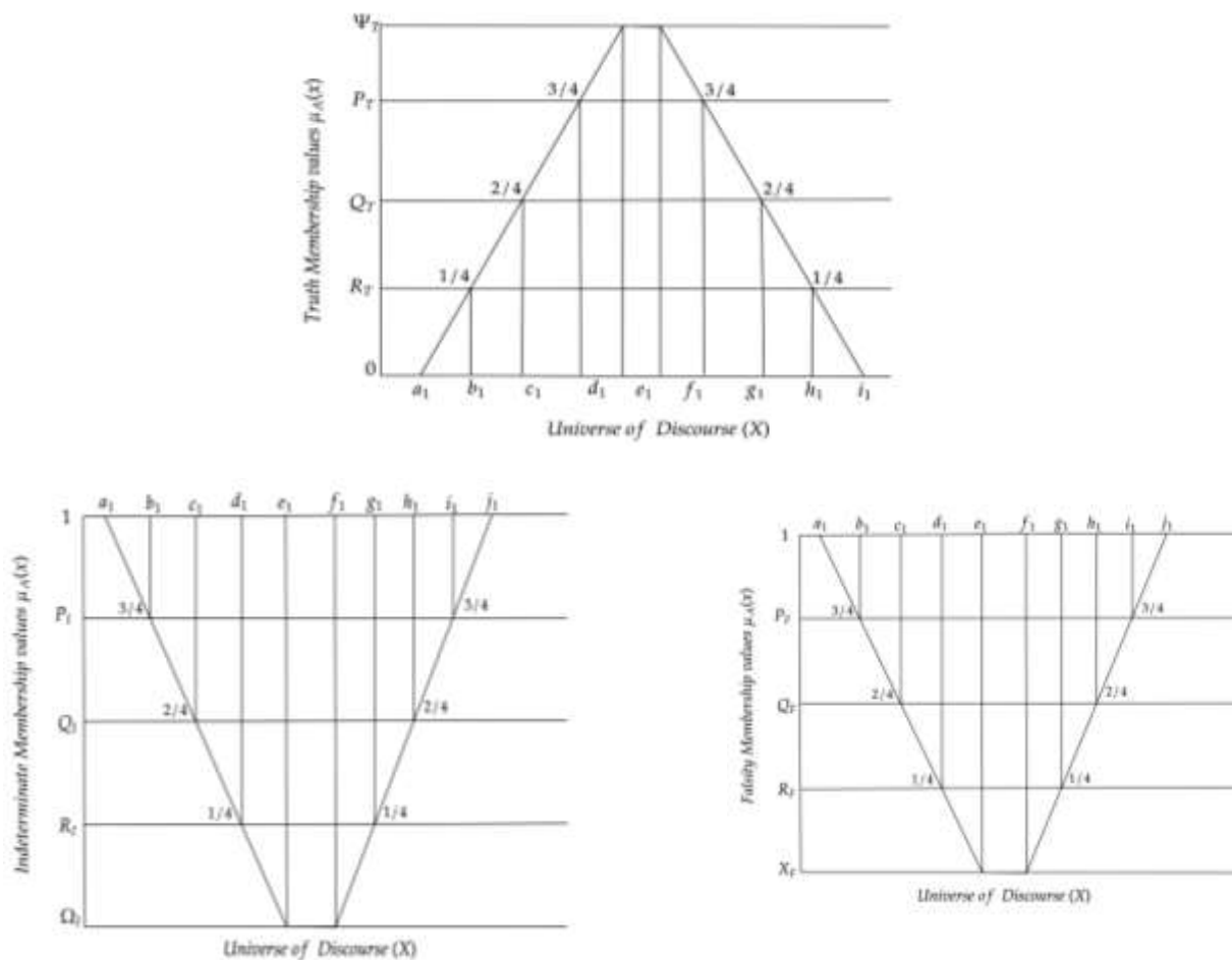
Figure 1 The Representation of special Decagonal Neutrosophic number Graphically
