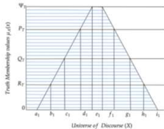
Figure 3: Right side area removal of
