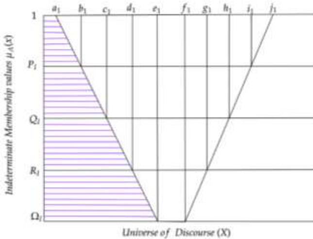
Figure 5: Right side area removal of Falsity
