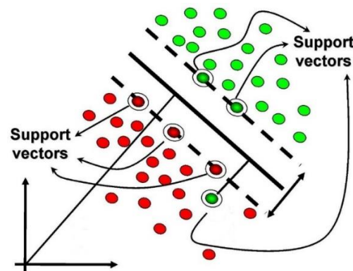
Figure 3: Structure of support vector machines.
