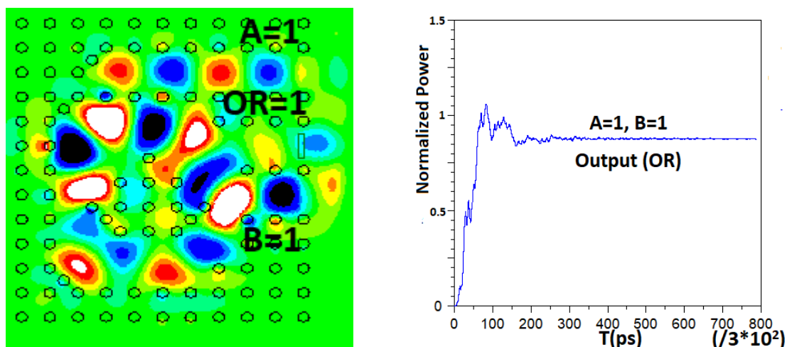
Figure 15: A = 1 and B = 1 (a) power distribution, (b) time response for 270-degree rotation
