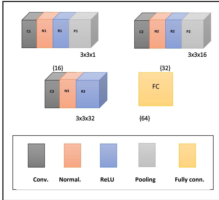
Figure 10: The proposed layers of DFNET
