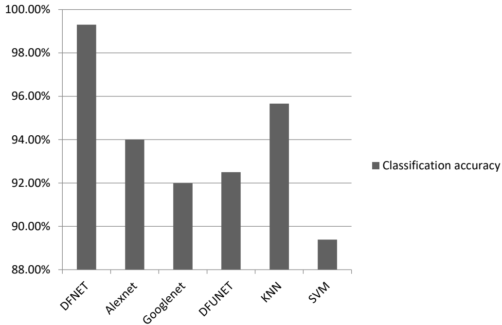
Figure 13: accuracy results of classifiers
