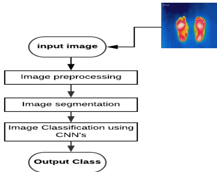
Figure 5: Thermal image analysis steps.
