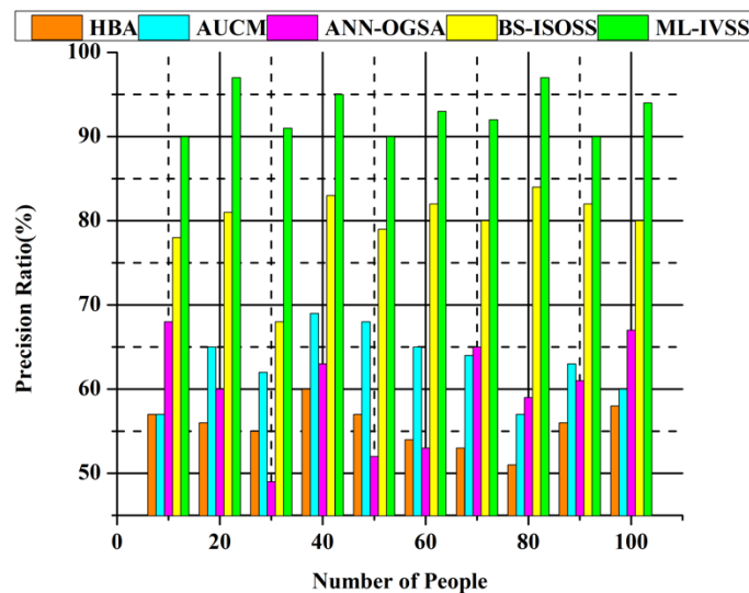
Figure 11: Precision Ratio
