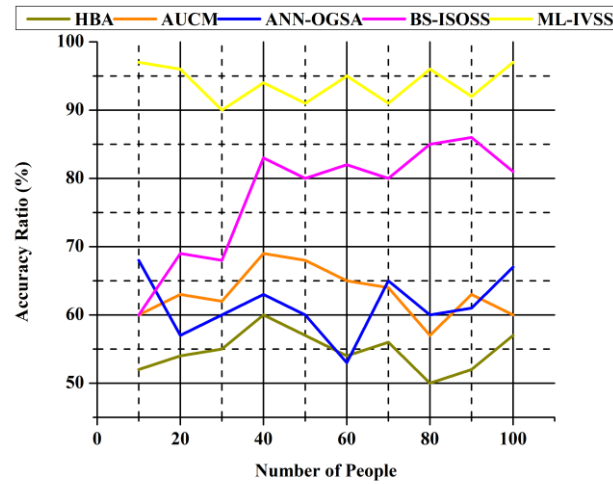
Figure 8: Accuracy Ratio
