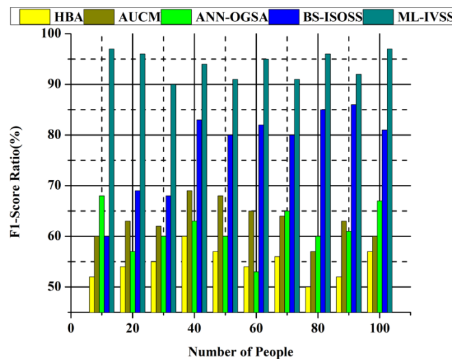
Figure 9: F1-Score Ratio
