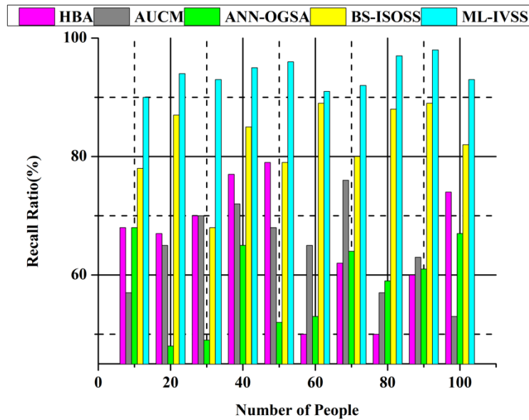
Figure 10: Recall Ratio
