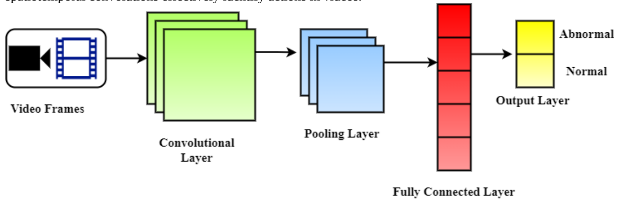
Figure 4: CNN Model
