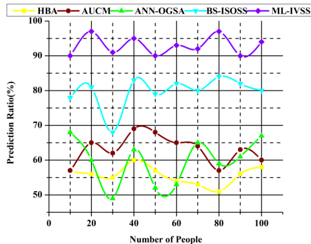
Figure 7: Prediction Ratio
