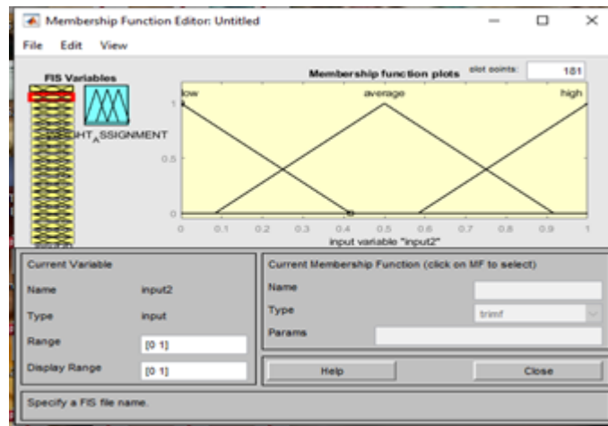
Figure 2: Membership Function
