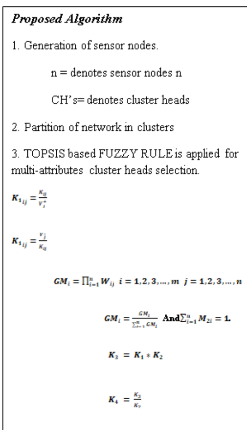
Figure 1: Proposed Algorithm
