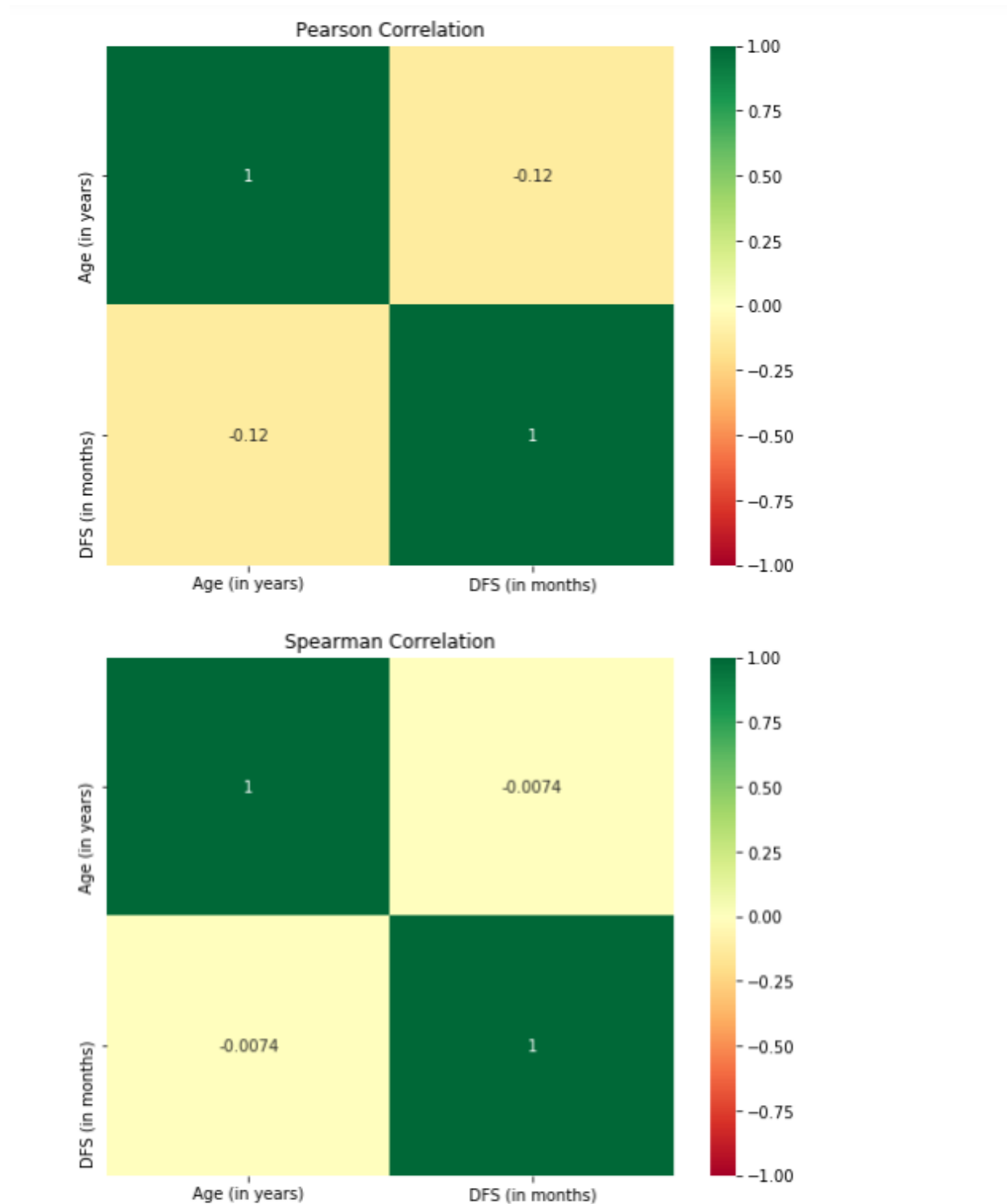
Figure 4: The Pearson and Spearman correlation between age and DFS.
