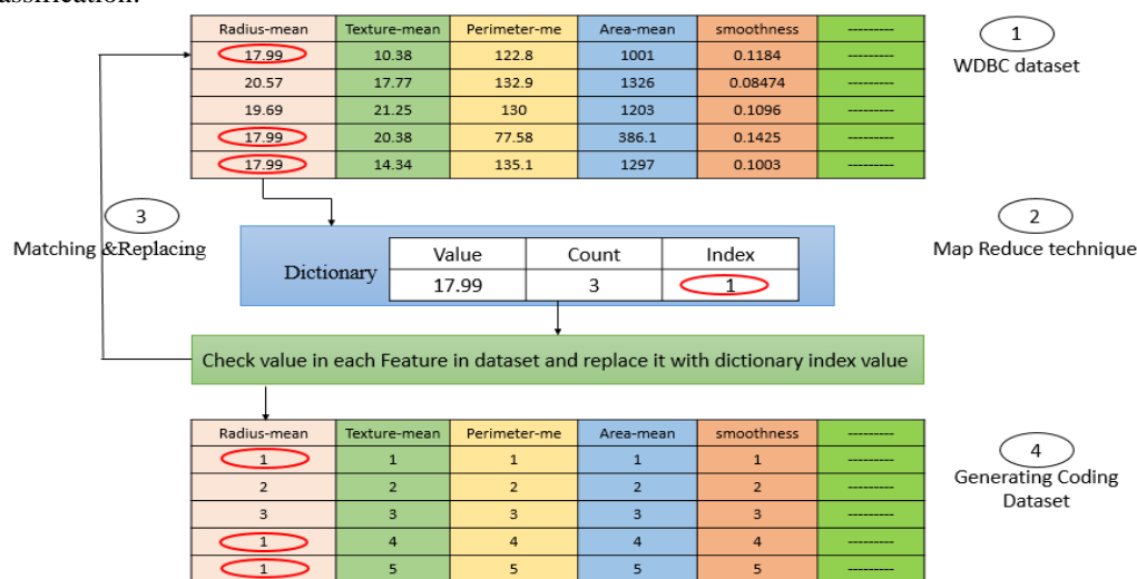
Figure 2: Main Steps of the Proposed Map-Reduce Technique to Generation Coding for Each Value in WDBC Dataset
