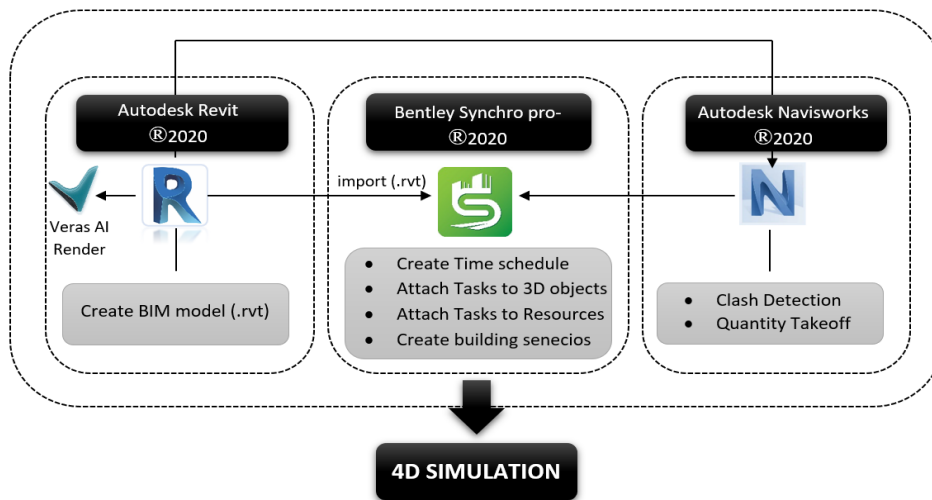
Figure 5: proposed workflow
