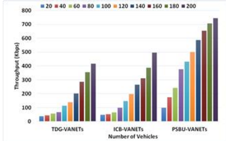
Figure 6: Throughput calculation
