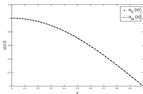
a) T=1 , \delta = 0
