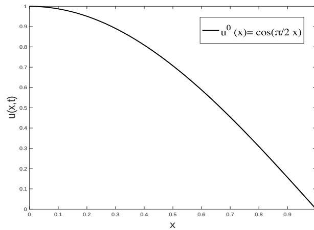
Figure 1: Initial condition u(x)
