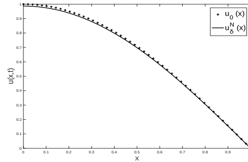
b) T=1 , \delta = 0.05
