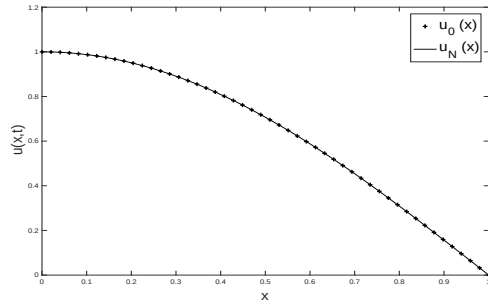
c) T=2, \delta = 0
