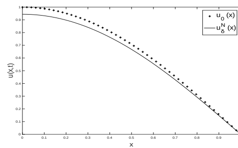
d) T=2, \delta = 0.05
