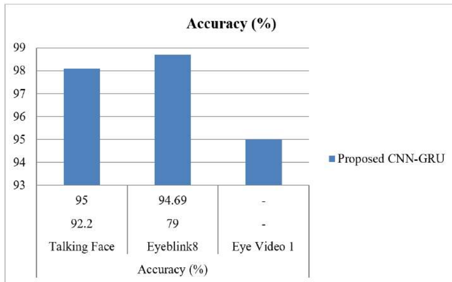
Figure 11: Accuracy Graph.
