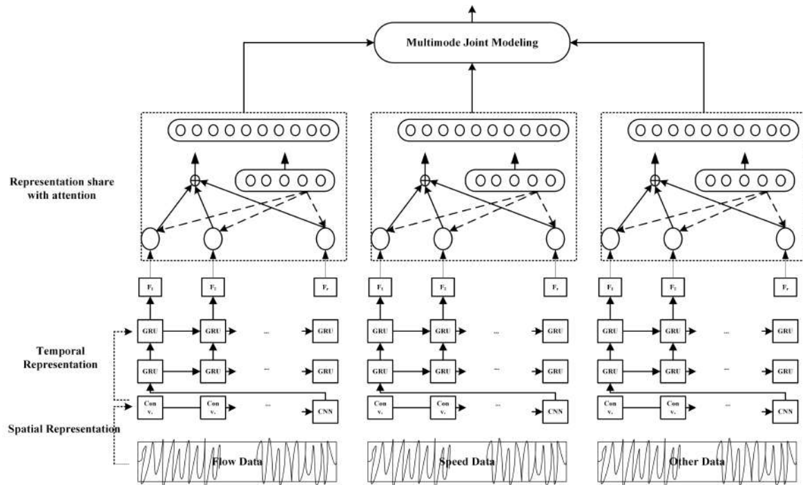
Figure 3: CNN-GRU Architecture.
