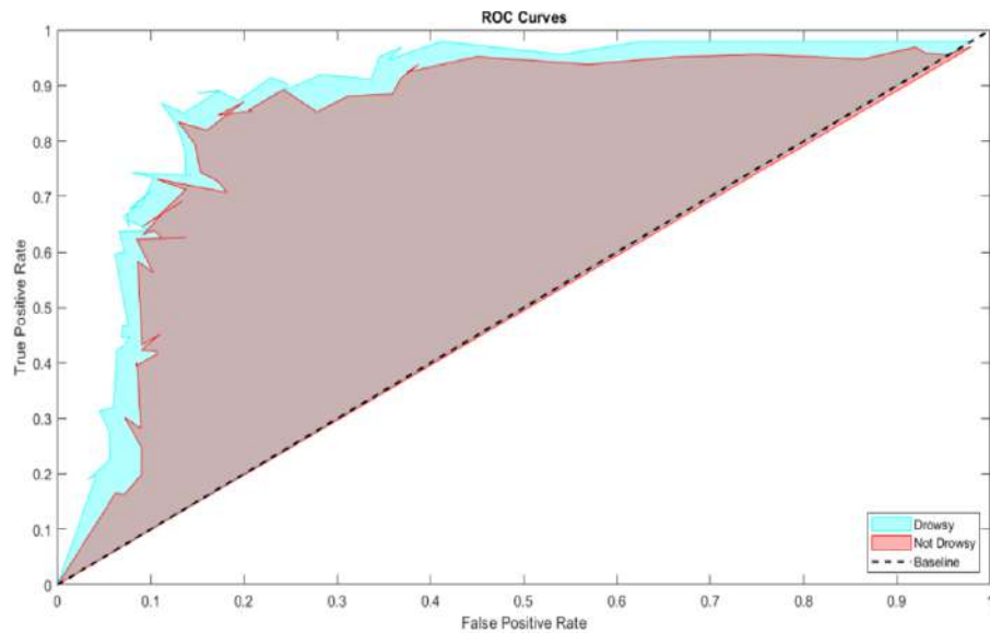
Figure 9: ROC curve.
