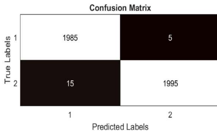
Figure 10: Confusion Matrix.
