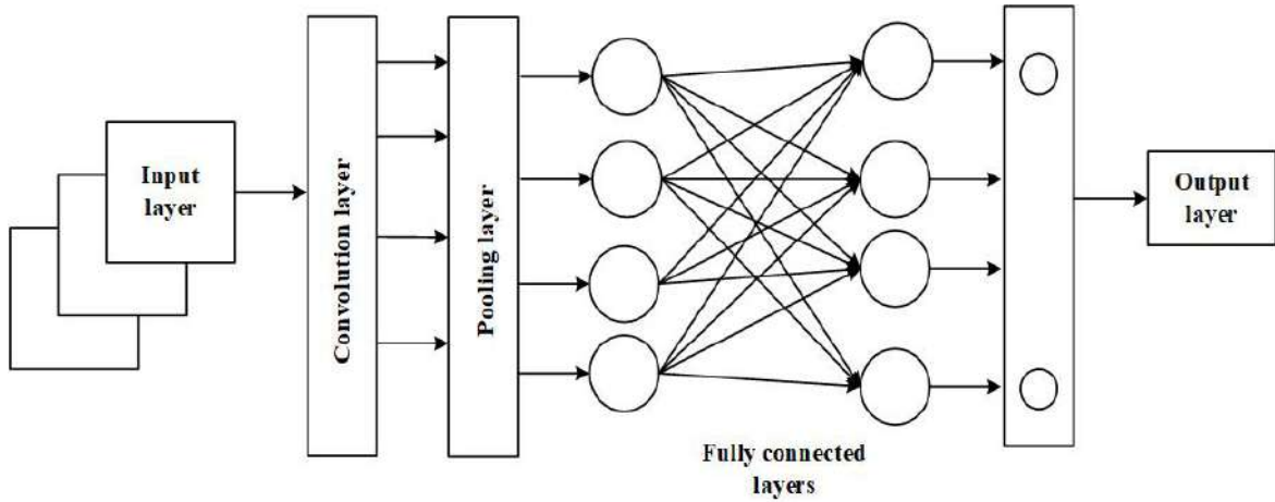
Figure 2: CNN Architecture.
