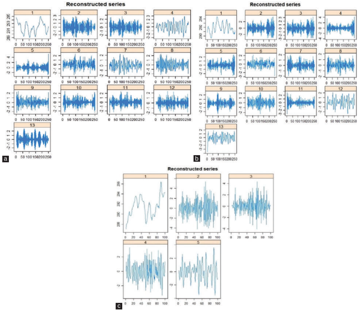
Figure 8: First stage: Elementary reconstructed series (a) dry season ( l=13 ), (b) rainy season ( l=13 ), and (c) inter-monsoon season ( L=5 ).
