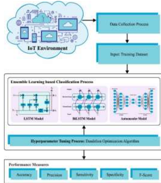
Figure 1: Workflow of AC-DOAEL methodology
