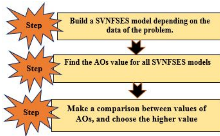
Figure 1: Algorithm
