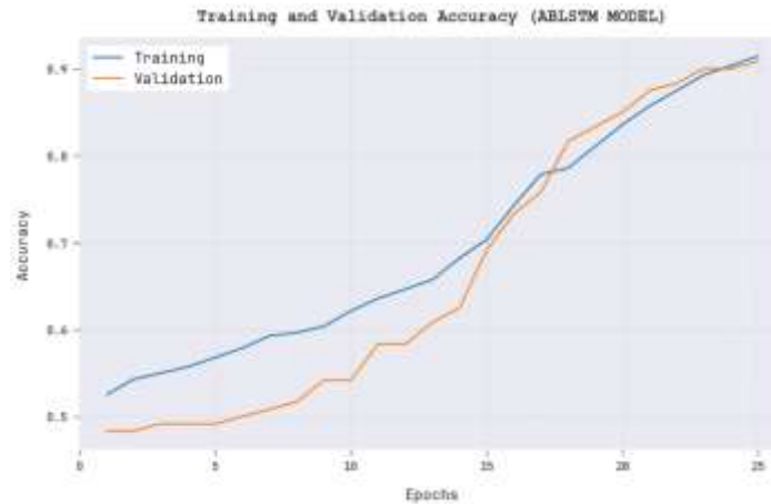
Figure 4: TR_{acc} and VL_{acc} analysis of ABLSTM method
