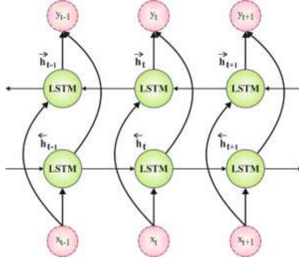
Figure 2: Structure of Bi-LSTM
