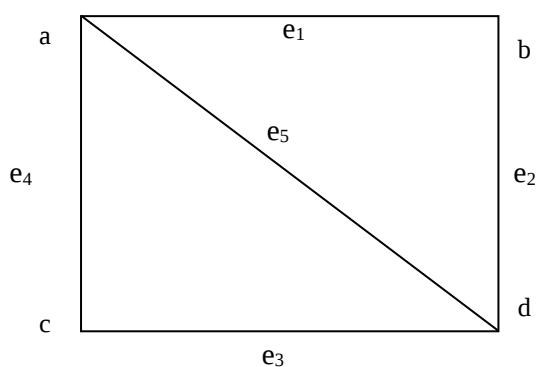
Figure 2: Graph of Incidency
