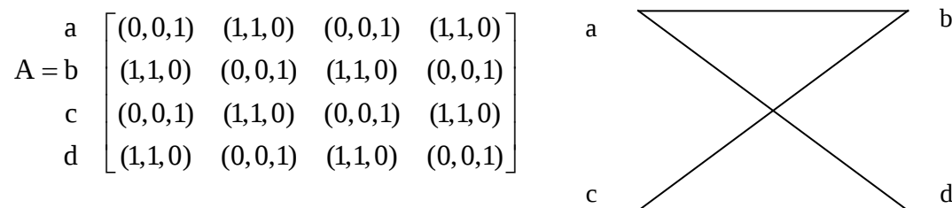
Figure 2: Graph of adjacency
