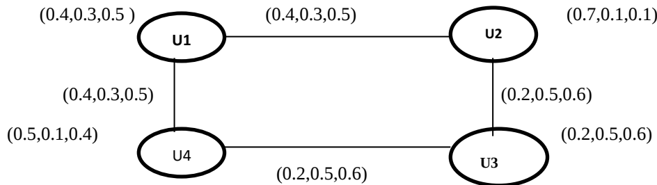
Figure 4: Strong single-valued neutrosophic graph
