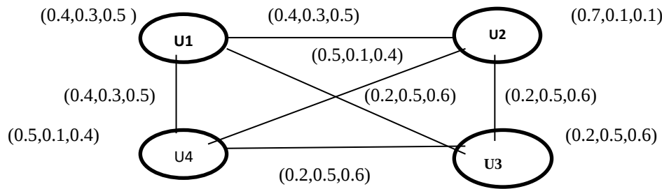
Figure 5: Complete- single valued neutrosophic – graph
