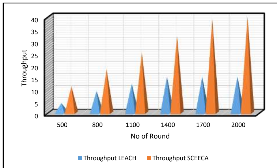
Figure 5: Throughput Evaluation of the Proposed Algorithm.
