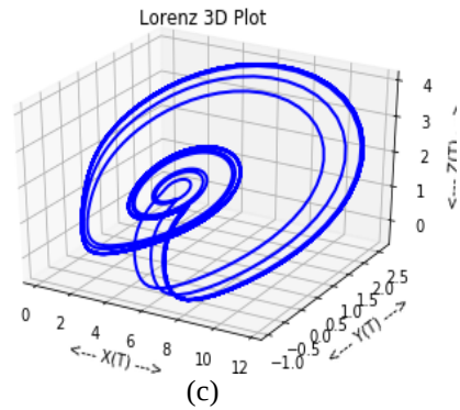
Figure 5: displays the various chaotic behavior for 3D multi-scroll systems under the initial conditions.
