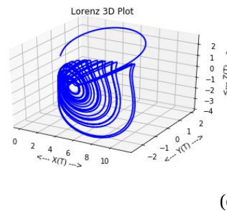
Figure 6: Chaotic Behaviour of the Proposed 3 D Hybrid Model with the Different Initial Conditions
