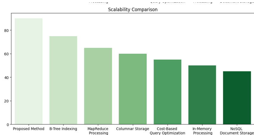
Figure 5: Scalability Comparison
