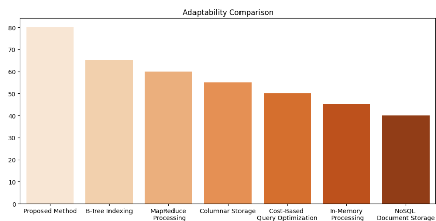
Figure 6: Adaptability Comparison
