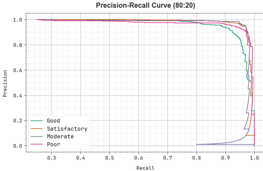
Figure 7: PR curve of the APMP-AVOAML technique under 80:20 of TRAS/TESS
