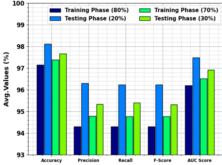
Figure 4: Average outcome of APMP-AVOAML technique
