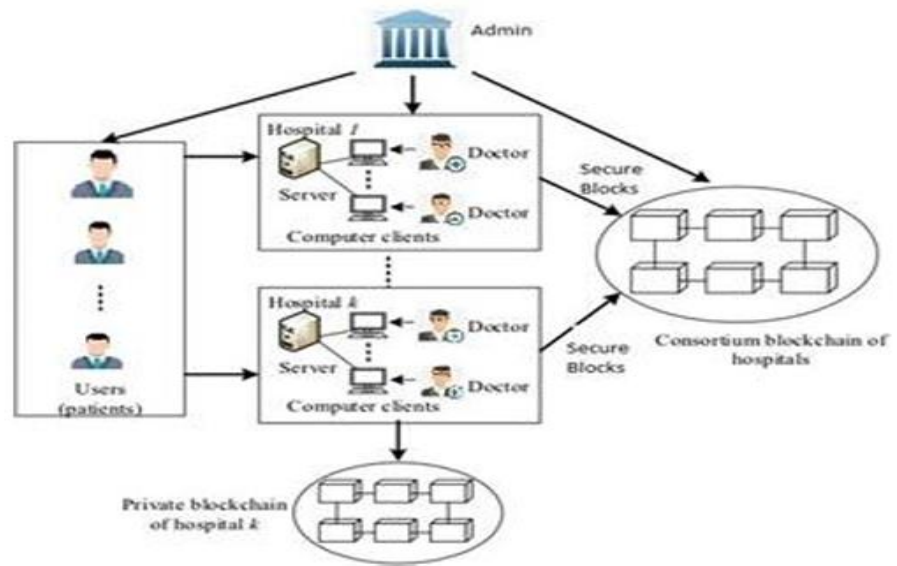
Figure 1: System Architecture
