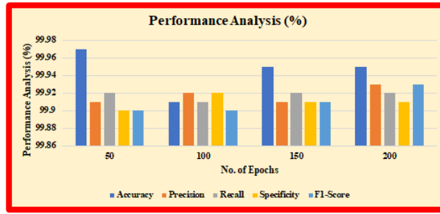
Figure 9: Performance metrics of proposed model utilizing the public health datasets
