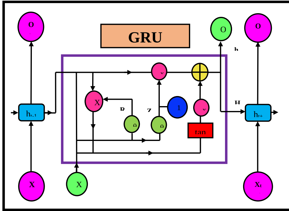
Figure 3: GRU -network Architecture
