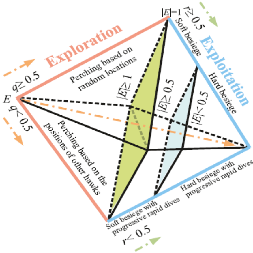
Figure 4: Different HHO phases
