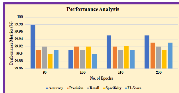
Figure 7: Performance metrics of proposed model utilizing the UCI Datasets
