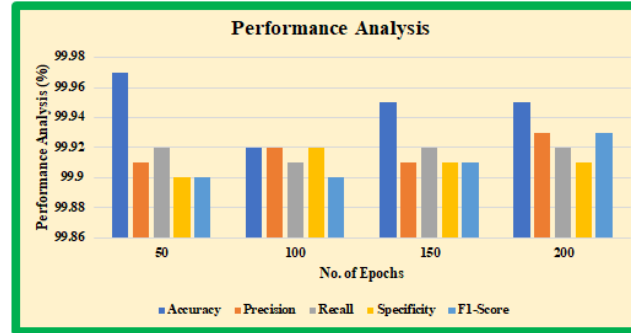
Figure 9: Performance metrics of proposed model utilizing the public health datasets
