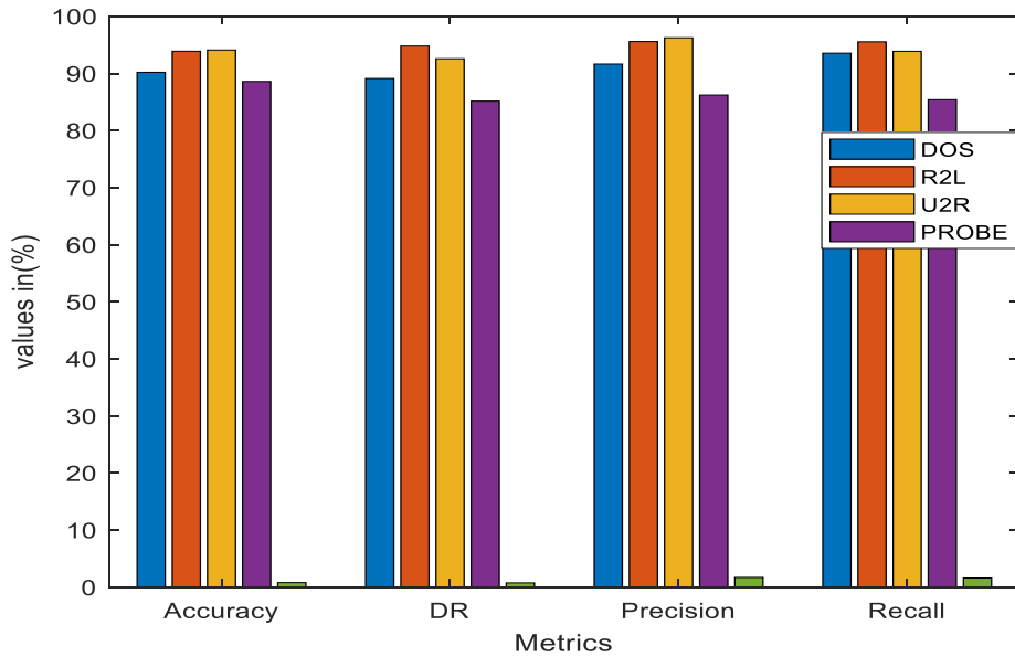
Figure 5. Performance metrics evaluation
