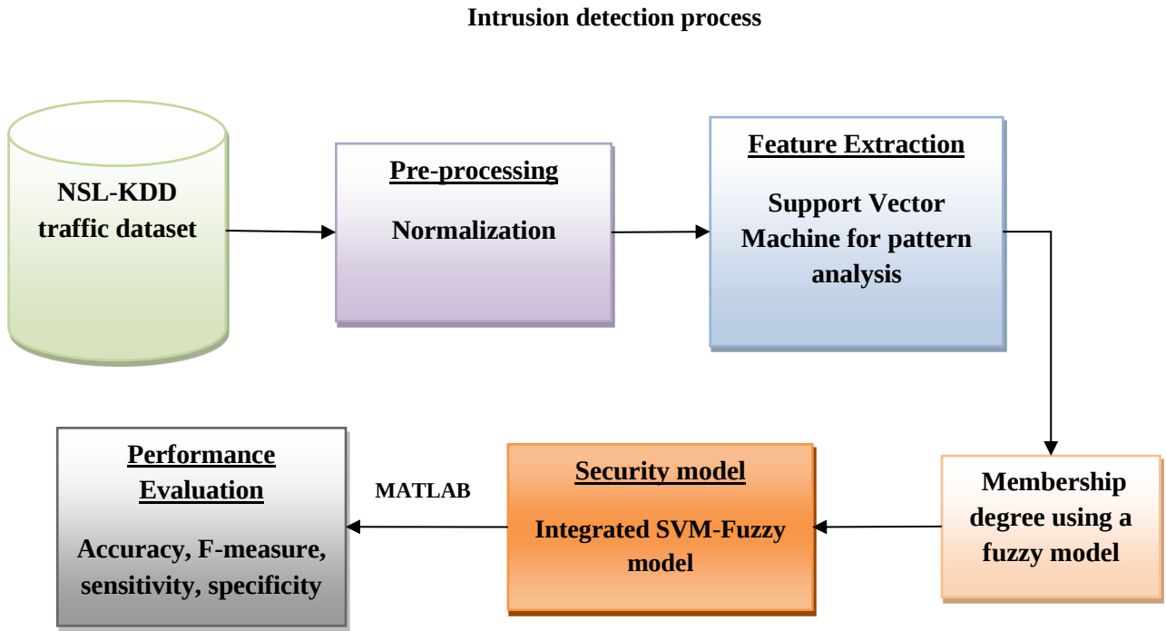
Figure 1. Block of the integrated fuzzy-SVM model
