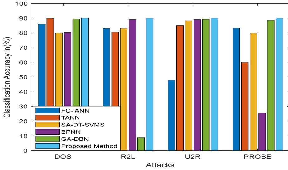
Figure 4. Evaluation of classification accuracy
