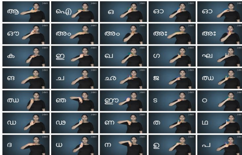
Figure 3. MSL Dataset
