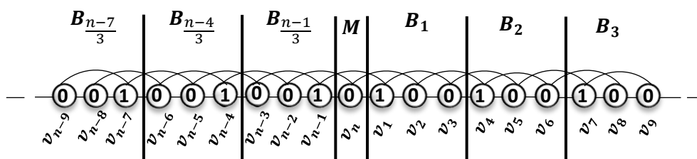
Figure 5. Applying configuration 10 on B_{\frac{n-1}{3}} \cup M \cup B_1 when n \equiv 1(mod 3) .
