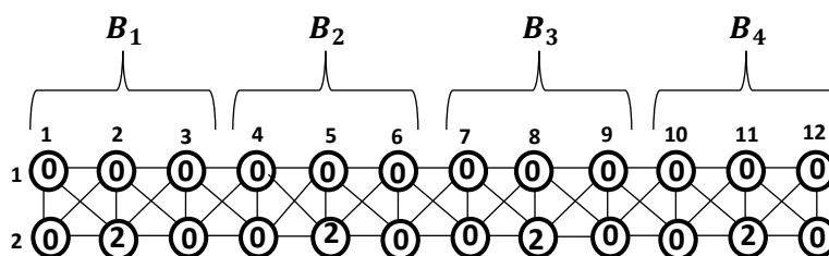
Figure 8. \gamma_l^p(P_2 \boxtimes P_{12}) \leq 8 .
