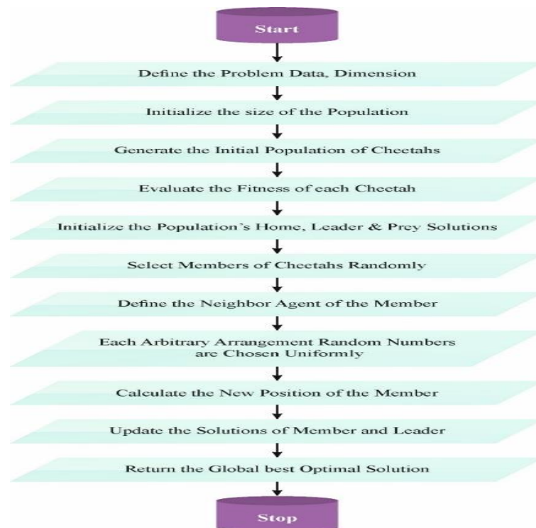
Figure 2. Flowchart of COA
