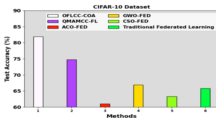
Figure 11. TACC analysis of the OFLCC-COA model on the CIFAR10 dataset
