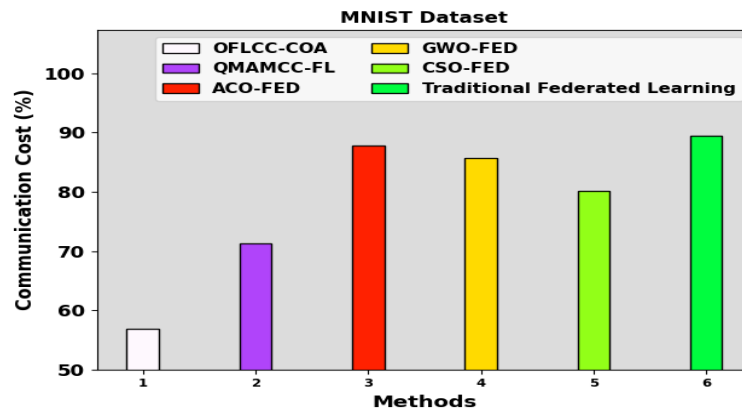
Figure 10. CC result of the OFLCC-COA method at MNIST dataset
