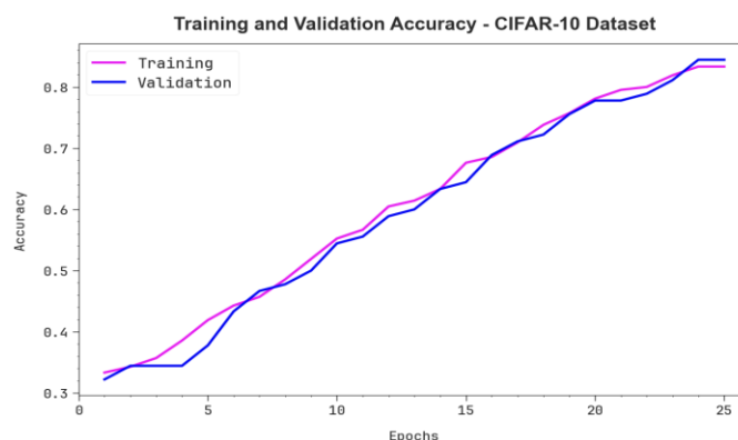
Figure 4. Accu_y curve of the OFLCC-COA system on the CIFAR10 dataset
