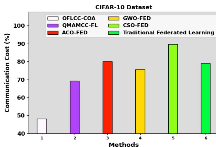
Figure 9. CC result of the OFLCC-COA system at CIFAR10 dataset
