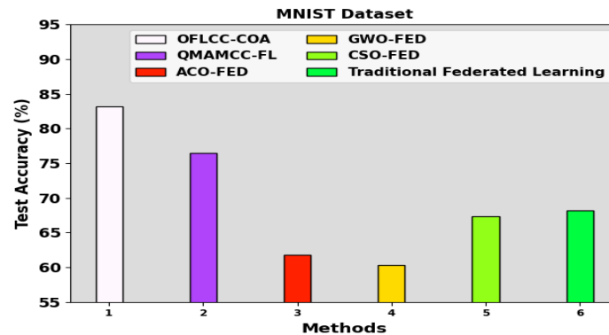
Figure 12. TACC outcome of the OFLCC-COA technique under the MNIST dataset
