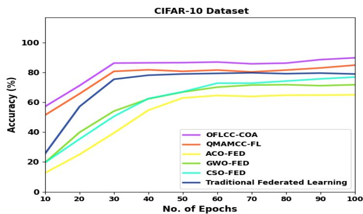
Figure 3. Accu_y Outcome of the OFLCC-COA technique at CIFAR10 dataset
