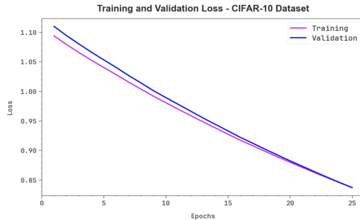
Figure 5. Loss curve of the OFLCC-COA algorithm under CIFAR10 dataset
