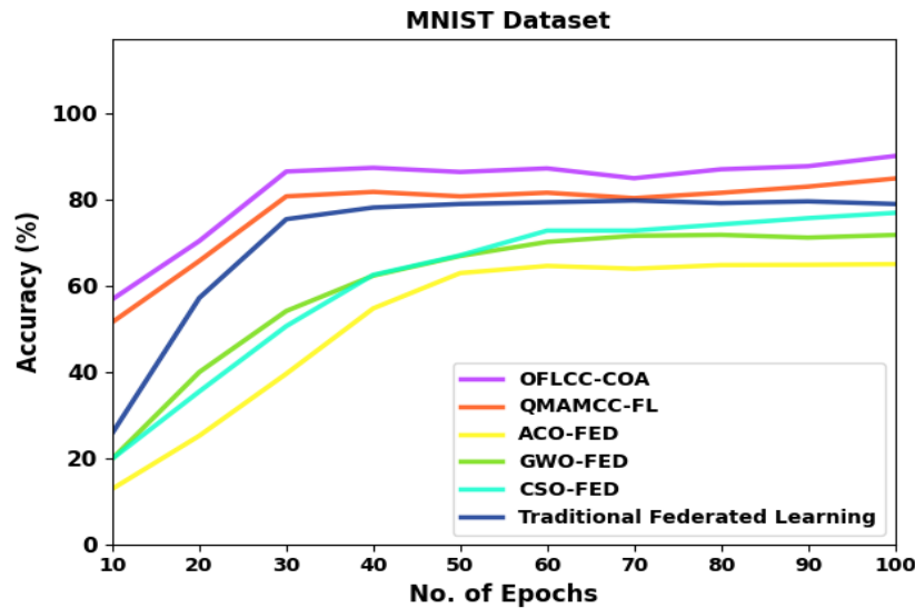
Figure 6. Accu_y Outcome of the OFLCC-COA system at MNIST dataset
