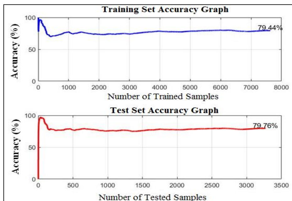
Figure 12. Training and Test Set Validation Graph.
