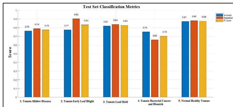
Figure 16. Test Data Set Classification Values.
