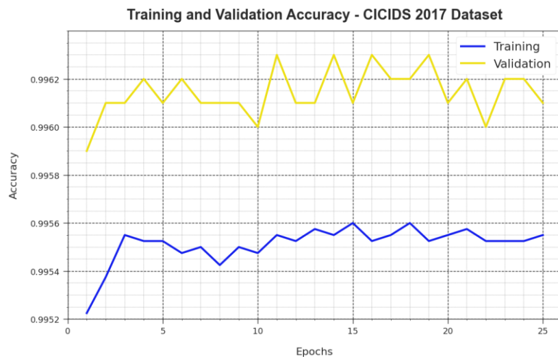
Figure 8. Accu_y Curve of the ATD-LOADL model under the CICIDS2017 dataset
