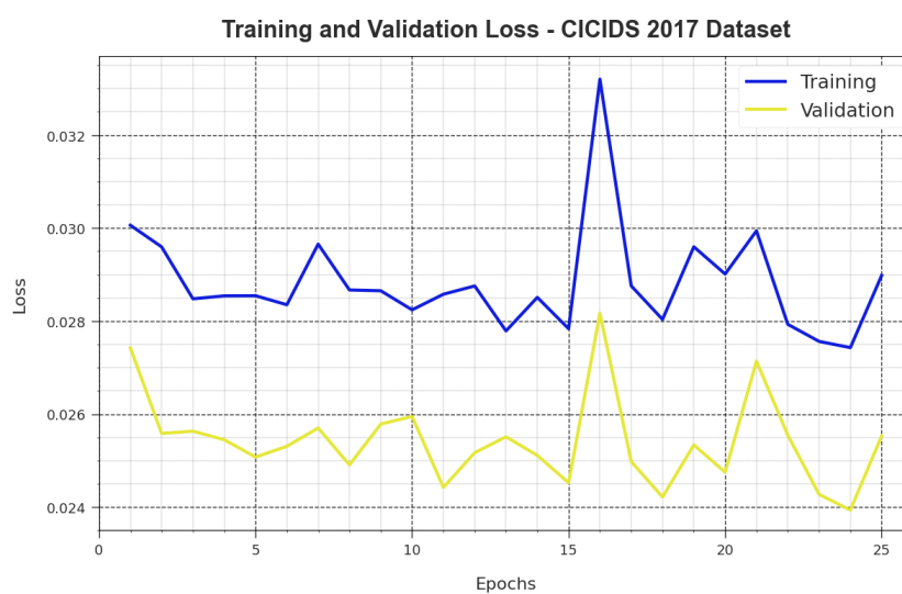
Figure 9. Loss curve of the ATD-LOADL technique with the CICIDS2017 dataset
