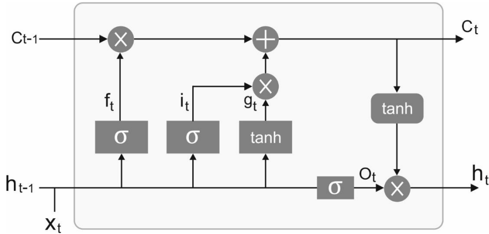
Figure 2. LSTM structure
