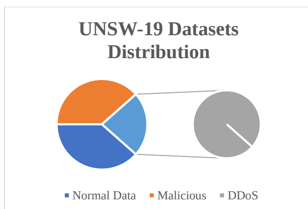
Figure 1. Datasets Distribution
