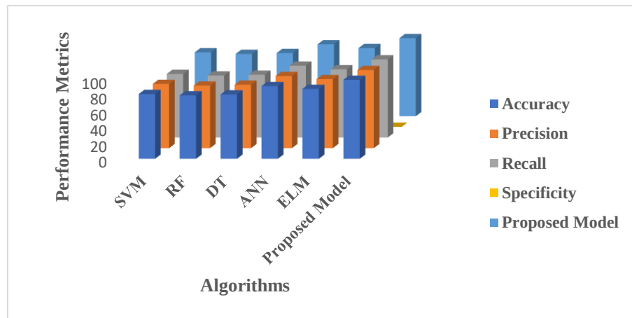
Figure 5. Correlative study of various Model for identifying the Normal Scenario (UNSW-19 Datasets)
