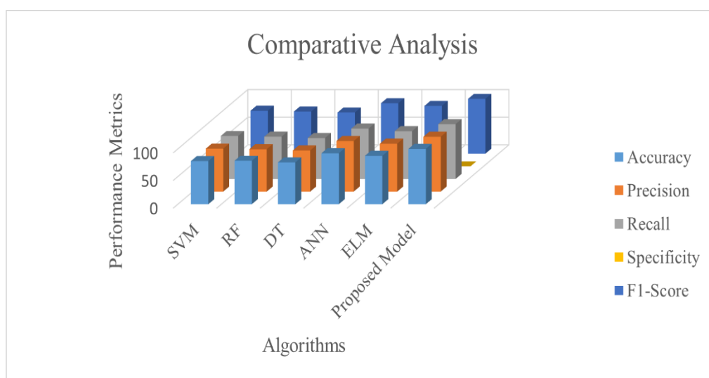
Figure 3. Correlative Study of various learning methodology in Normal Scenario (NSL-KDD Datasets)
