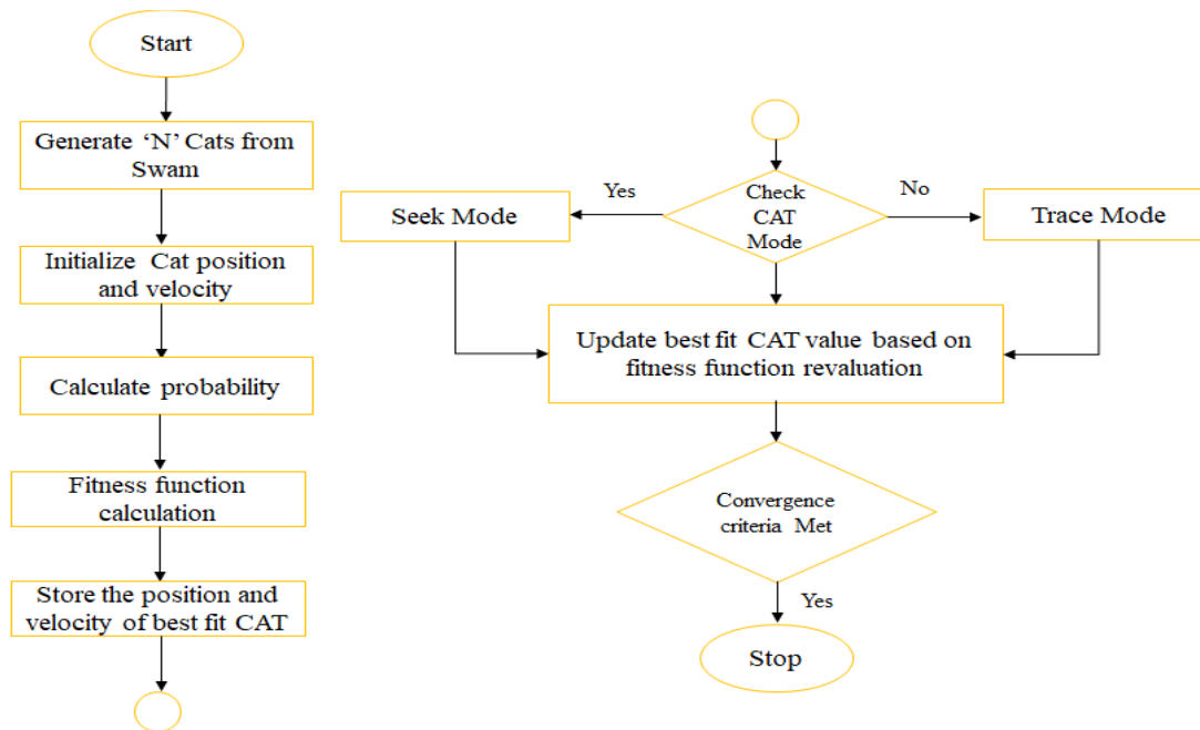
Figure 2. Comprehensive schematic illustration for the cat swarm Methodology
