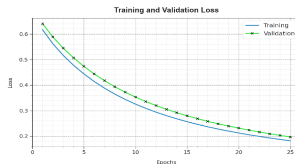
Figure 5. Loss curve of FCRF-BSVNGSA model
