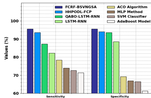
Figure 6. sens_y and Spec_y outcome of FCRF-BSVNGSA technique with existing models
