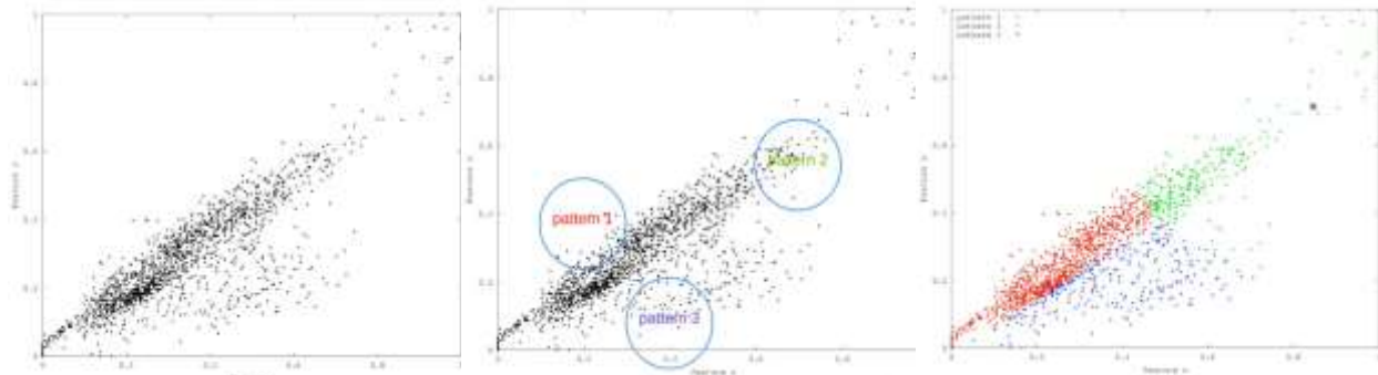
Fig 2. Supervised Classification
