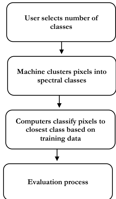
Fig 3. Unsupervised Classification
