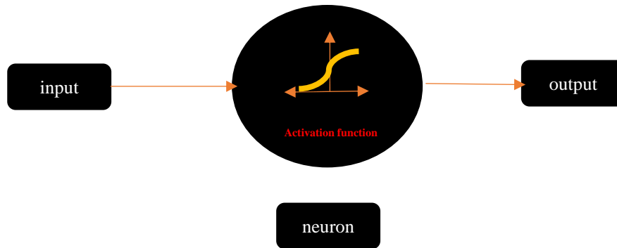
Fig 20. Activation functions.
