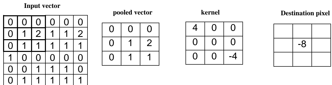
Figure 26.A visual representation of a convolutional layer. The center component in The kernel is placed over the input vector, which is then calculated and replaced By a weighted sum of itself and any nearby pixels.
