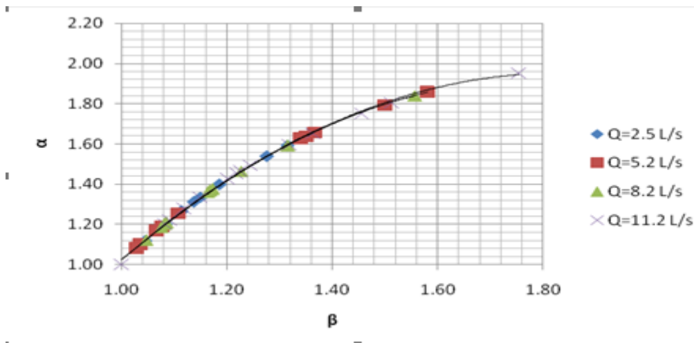
Figure 4: Relationship between \alpha and \beta at upstream section
